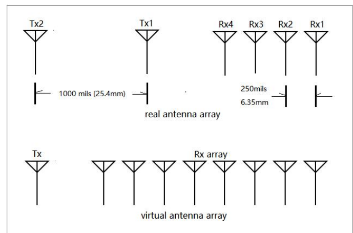
Figure 2. Antenna array
